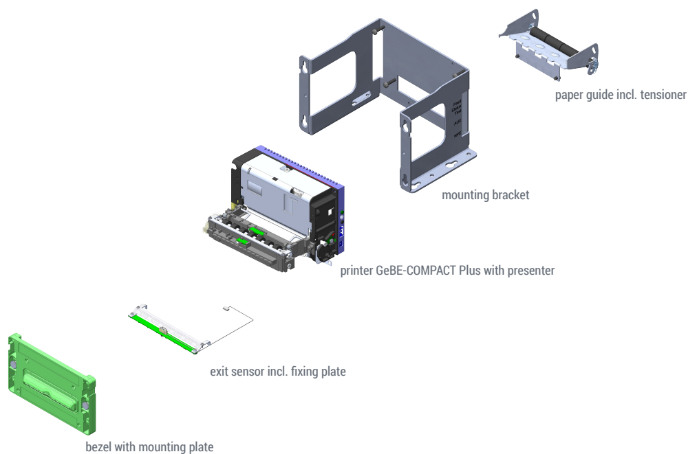
Figure 2: Possible combination of GeBE-COMPACT Plus GPT-467x with presenter and paper guide
