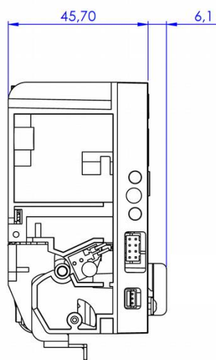
Side view from the right
