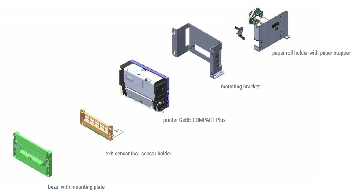
Figure 1: Possible combination of GeBE-COMPACT Plus GPT-467x with paper roll holder
